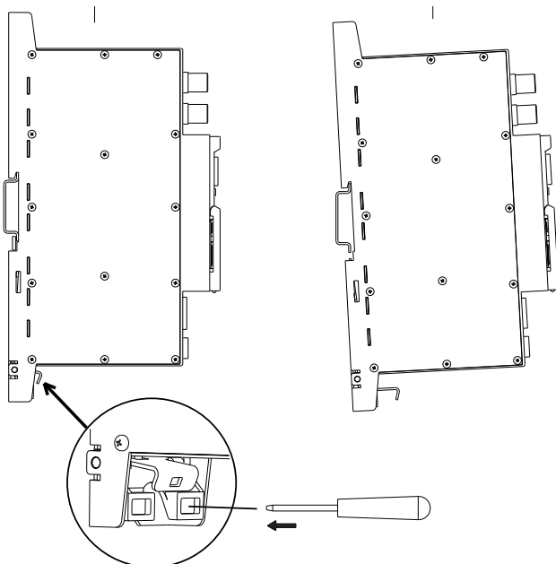
Figure 4. Mounting from DIN rail
