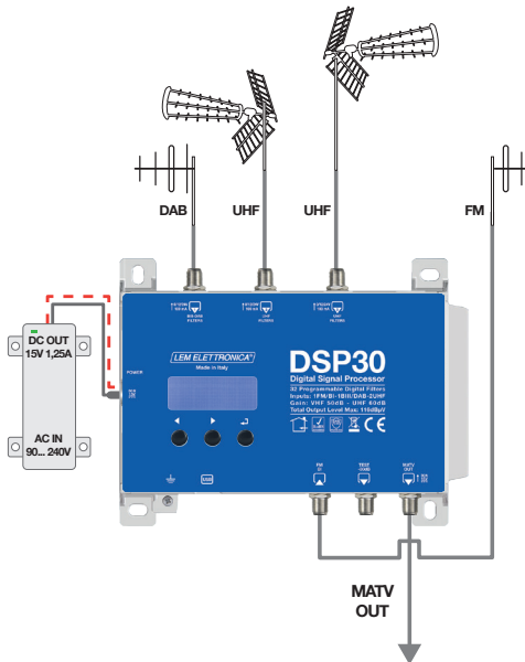
DSP30 power supply through the DC input.
