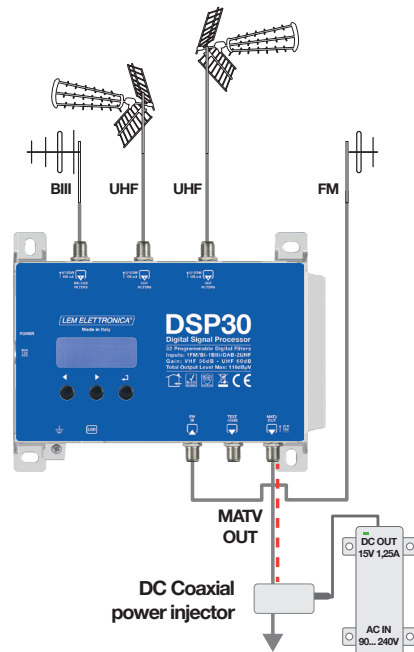
DSP30 power supply through the SMATV OUT.
