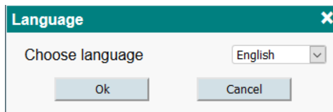
Figure 28. Language selection
